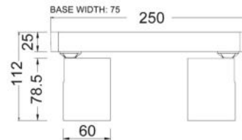
SPOT-BAR2B
