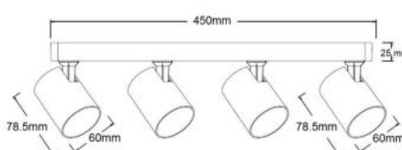
SPOT-BAR4B
