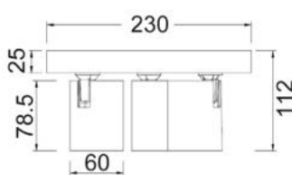
SPOT-R3B
