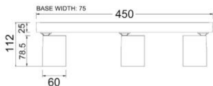
SPOT-BAR3B
